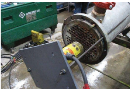
TUBE BUNDLE REMOVAL FOR REPAIR OR SERVICE
